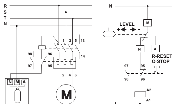
WIRING DIAGRAM FOR EMPTYNG PUMP
