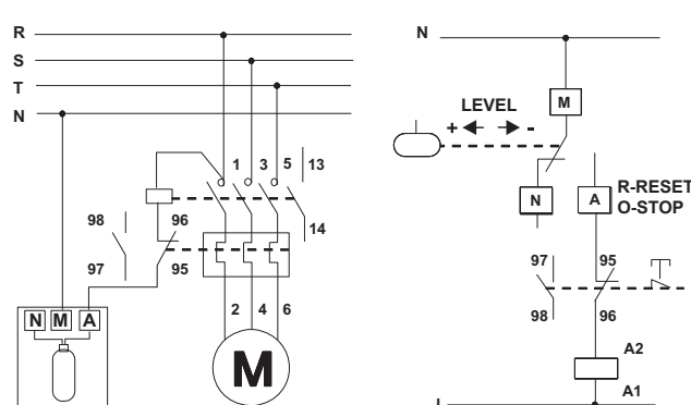
WIRING DIAGRAM FOR FILLING PUMP
